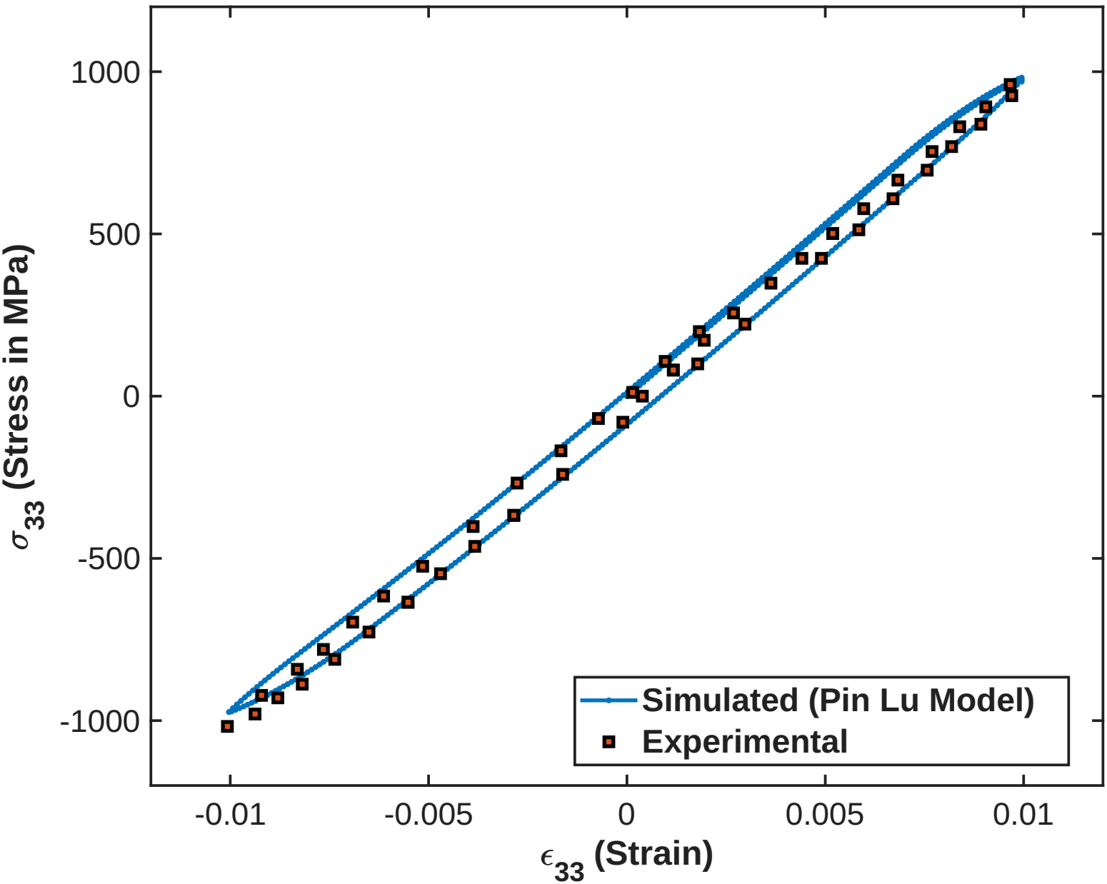
Cyclic Test upto 1% strain
